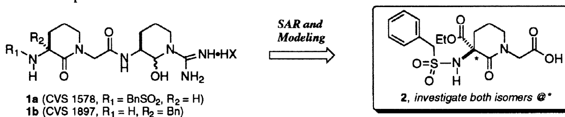
Figure 1: Design of quaternary lactam advanced intermediate 2 .
