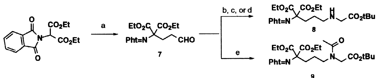
Scheme 2: Reagents and Conditions: (a) 1. Acrolein, \text{DIPEA} , \text{EtOH} , 0^\circ\text{C} to rt, 3 d; 2. \text{HOAc} , 72 %, 20–25 g scale or 1. \text{NaOEt} (cat.), \text{EtOH} , 0^\circ\text{C} to rt, 1 d; 2. \text{HOAc} , 38%, 5–10 g scale; (b) 1. \text{HCl}\cdot\text{GlyO-tBu} , \text{Et}_3\text{N} , \text{EtOH} , rt; 2. \text{H}_2 , \text{Pd/C} , 1 atm, ~27–40%; (c) \text{HCl}\cdot\text{GlyO-tBu} , \text{NaCNBH}_3 , \text{EtOH} , rt, 79 %; (d) \text{HCl}\cdot\text{GlyO-tBu} , \text{Na(OAc)}_3\text{BH} , \text{DCE} , \text{Et}_3\text{N} , rt, 65–68%, 9–15 g scale; (e) \text{HCl}\cdot\text{GlyO-tBu} , \text{Na(OAc)}_3\text{BH} , \text{DCE} , \text{Et}_3\text{N} , rt to 50^\circ\text{C} to reflux, 7 d, 44%.
