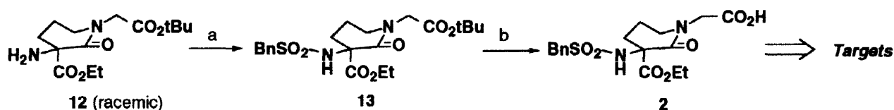
Scheme 4: Reagents and Conditions: (a) \text{BnSO}_2\text{Cl} , \text{Et}_3\text{N} , DMAP, \text{CH}_3\text{CN} , 0^\circ\text{C} to rt, 62%; (b) TFA, \text{CH}_2\text{Cl}_2 , 0^\circ\text{C} to rt, 82-85%
