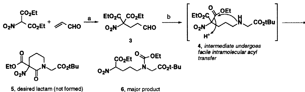
Scheme 1: Reagents and Conditions: (a) 1. \text{NaOEt} (cat.), \text{EtOH} , rt; 2. \text{HOAc} , 71%, 9 g scale; (b) \text{HCl}\cdot\text{GlyO-tBu} , \text{Na(OAc)}_3\text{BH} , \text{DCE} , \text{Et}_3\text{N} , \text{HOAc} , rt, 61% or \text{HCl}\cdot\text{GlyO-tBu} , \text{NaBH}_4 , \text{Et}_3\text{N} , \text{MeOH} , rt to 50^\circ\text{C} , 18 hr, ~85%.
