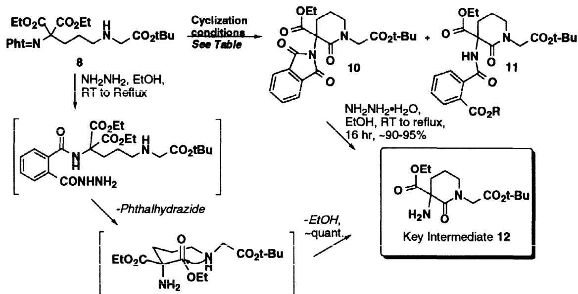
Scheme 3: Cyclization studies to key intermediates 10 and 12 . See Table 1 and text.
